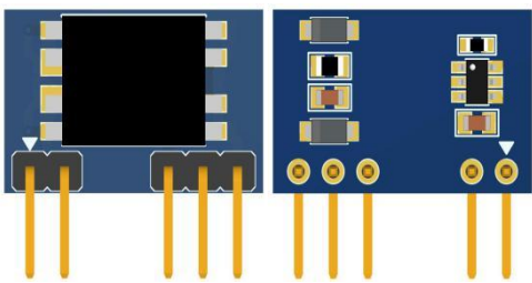
图 1: VPS8702B Demo 板 (19mm*12mm)
