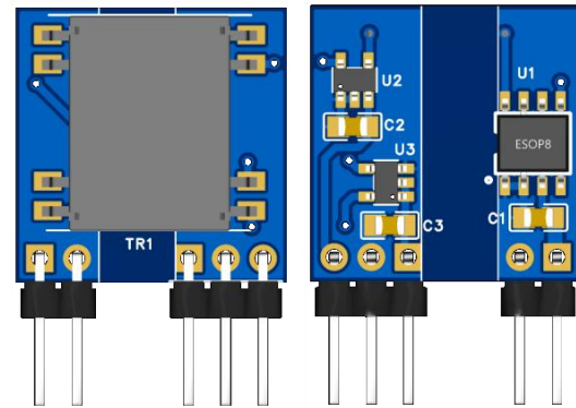
图 1: 尺寸: 18.5mm*18.8mm
