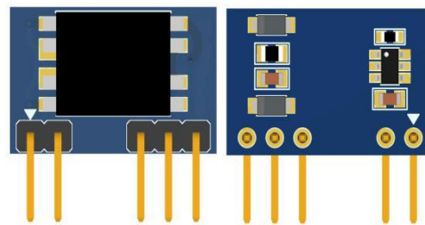
图 1: VPS8701B Demo 板 (19mm*15mm)
