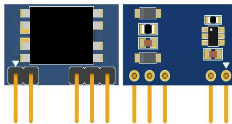
图 1: VPS8702 Demo 板 (19mm*12mm)
