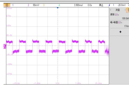
VIN=5.5V, 75%-50%-75%Io 动态波形
